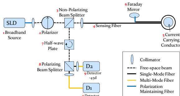
Figure 3. Faraday sensor setup.
