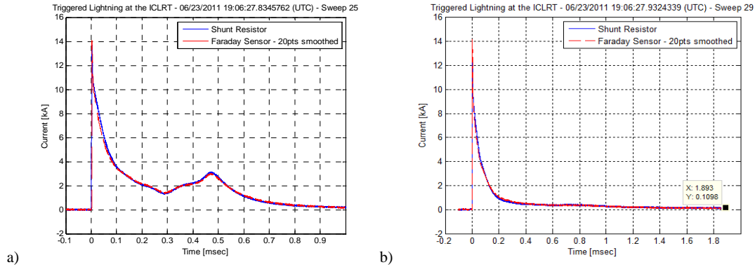
Figure 12. Results comparison for two strokes in the first lightning flash.
