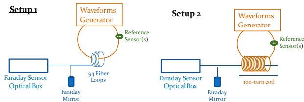
Figure 6. Using multiple fiber loops or a coil winding to simulate effects due to higher current.
