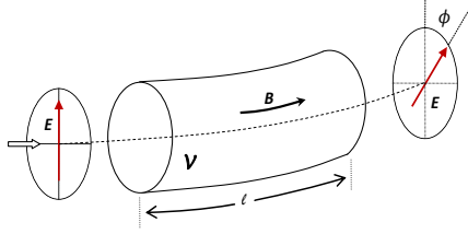
Figure 2. Faraday rotation in optical fiber.
