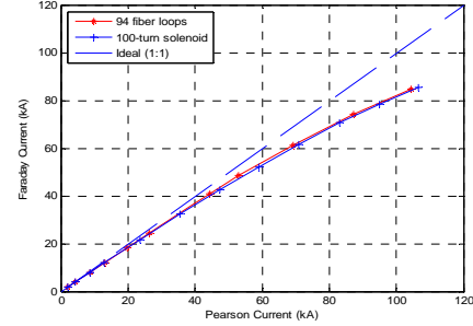
Figure 7. Response functions for two setups.
