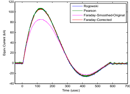
Figure 9. Faraday sensor comparison against reference sensors for a 110 kA peak current waveform.
