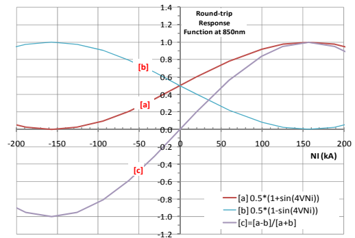
Figure 5. Reflective scheme response functions at 850 nm.
