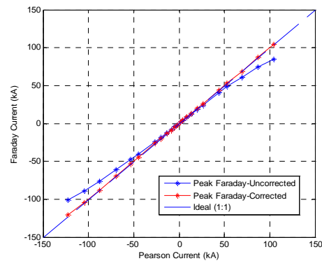
Figure 8. Faraday sensor’s uncorrected and corrected (linearized) response curves.
