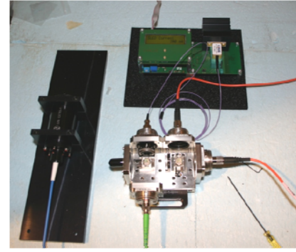
Figure 4. Key components: Faraday mirror (left), laser (top), and optical fiberbench (bottom right).
