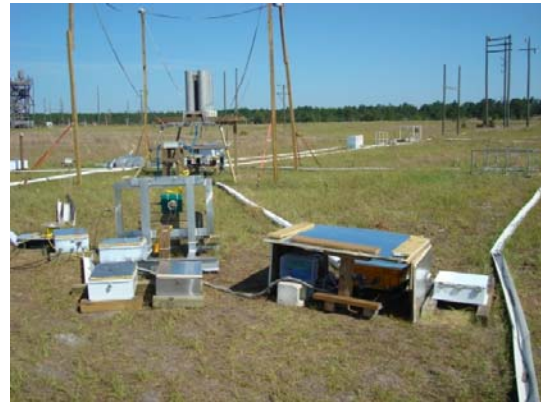
Figure 10. Field setup (right) located 12 m from the rocket launch pad.
