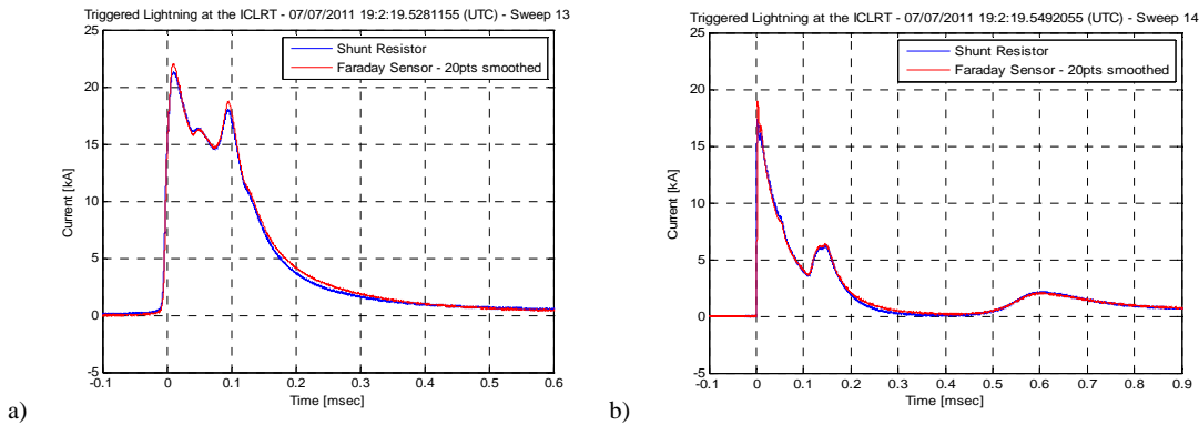
Figure 13. Waveform comparison in subsequent measurements. Faraday sensor data scaled to 90%.
